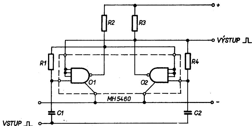
Fig. 44. Bi-stable flip-flop
