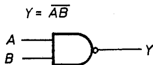
Fig. 45. Logical product
